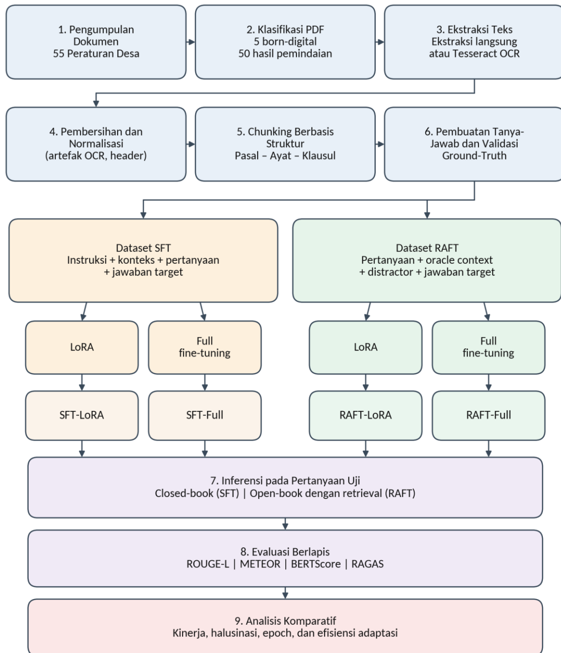
Gambar 1 Alur penelitian
