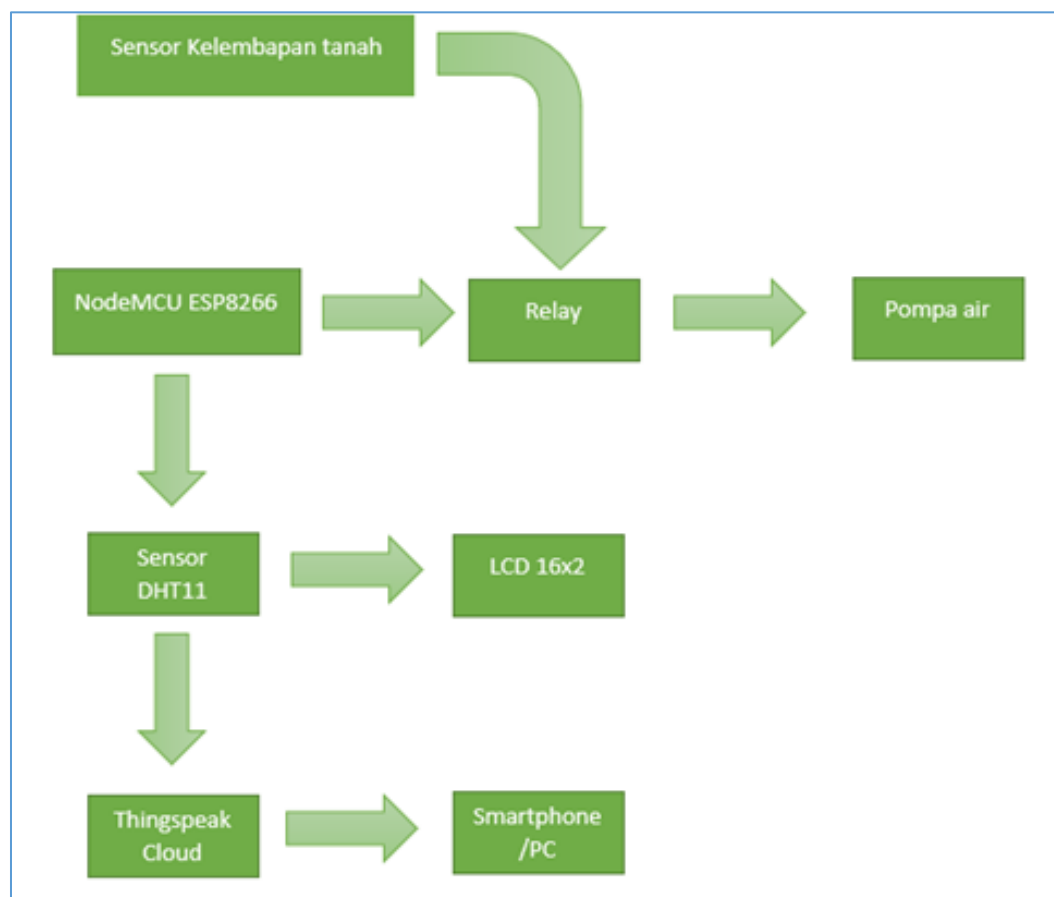
Gambar 1 Diagram alur sistem monitoring tanaman tomat
