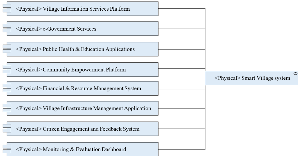
Figure 6. Application Communication Diagram
